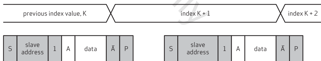
figure 2-15 SCCB single read from current location
