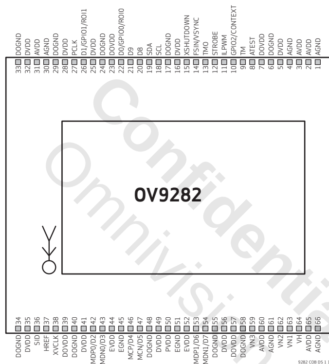
figure 1-1 pad diagram
