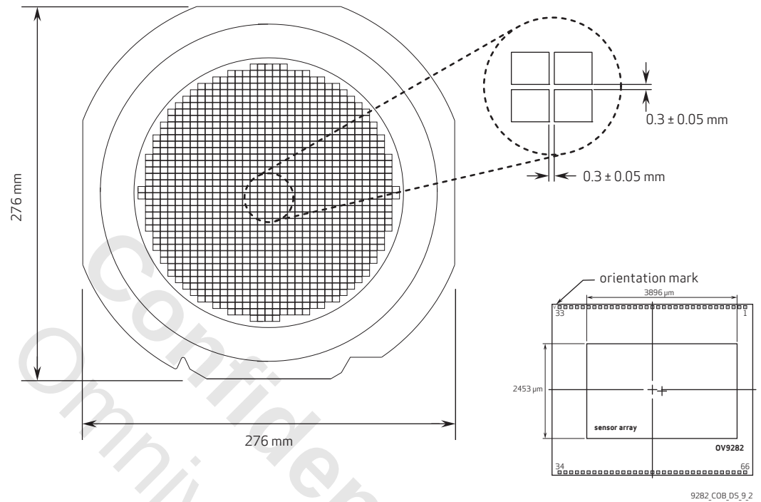
figure 9-2 OV9282 RW physical diagram
