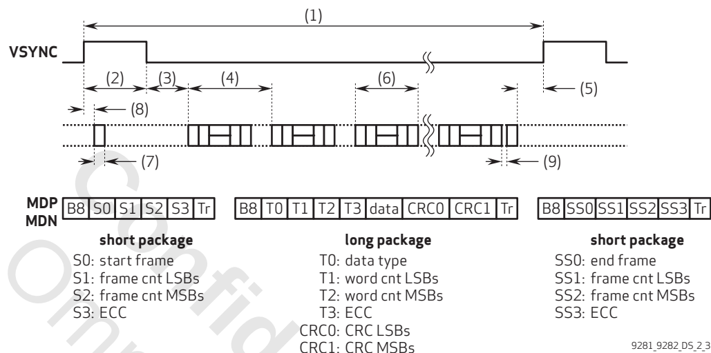
figure 2-3 MIPI timing
