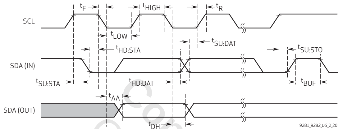
figure 2-20 SCCB interface timing
