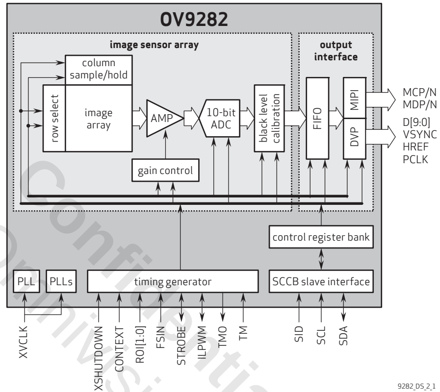
figure 2-1 OV9282 block diagram
